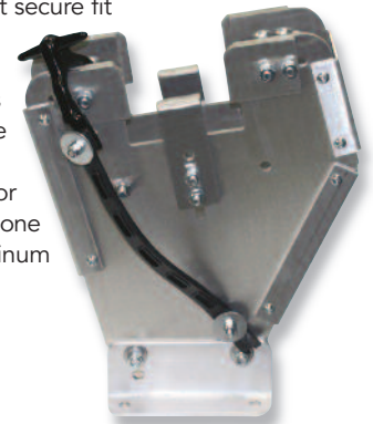
BL466 Multiversal Extrication Tool Holder
