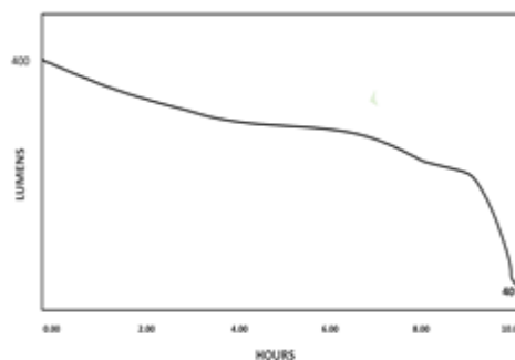
PERFORMANCE CURVE
