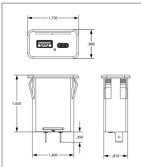
OUTLINE DRAWING
